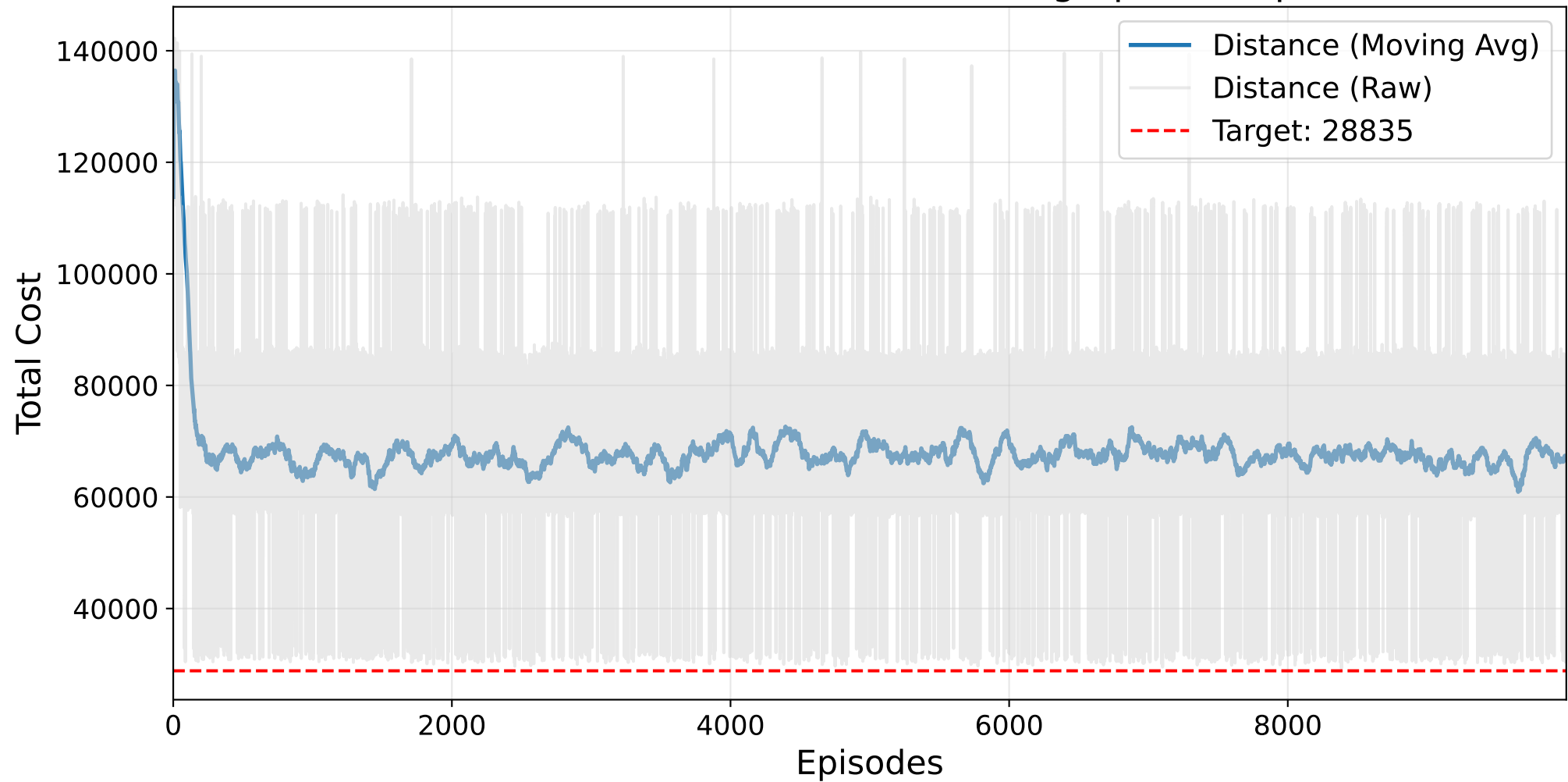
Final Masked AutoRL-SOP Training - p43.3.sop
